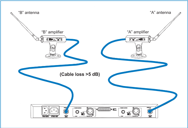
Antenna amplifiers
