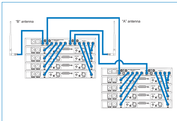
Antenna distribution: 8 receivers (master/slave)
