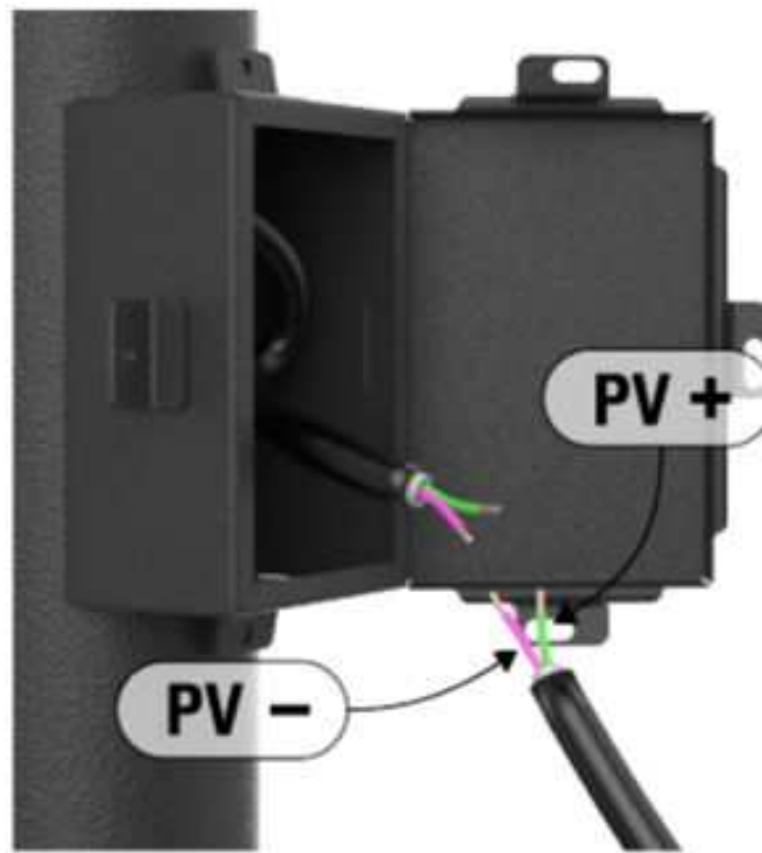
Figure 15: Conductors Connection
