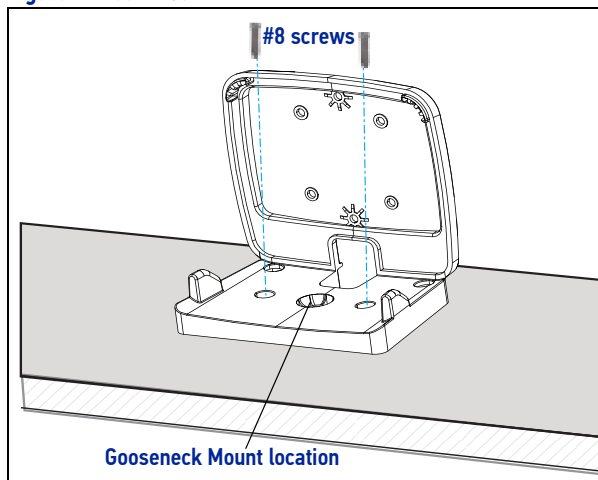
Figure 7. Desk Mount
