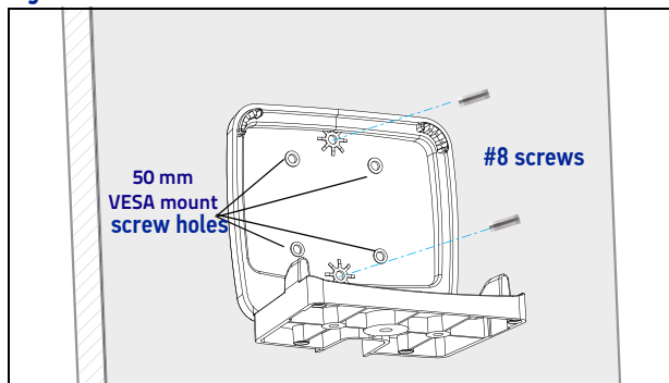
Figure 9. Wall mount
