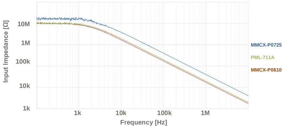
Typical Differential Input Impedance – MMCX-P0725, MMCX-P0610(RO)
