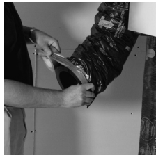
Finish by taping the vapor barrier to the collar to insure proper seal.
