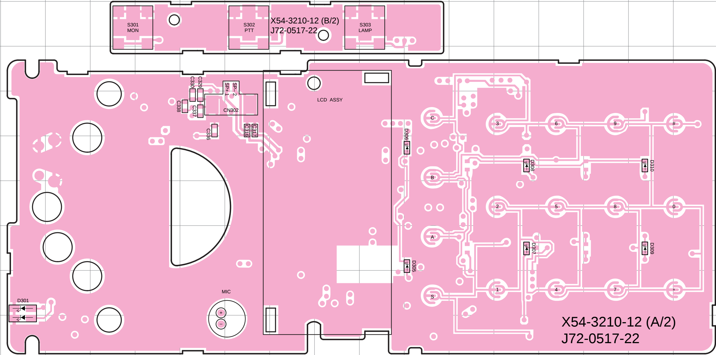
DISPLAY UNIT (X54-3210-12) Component Side View
