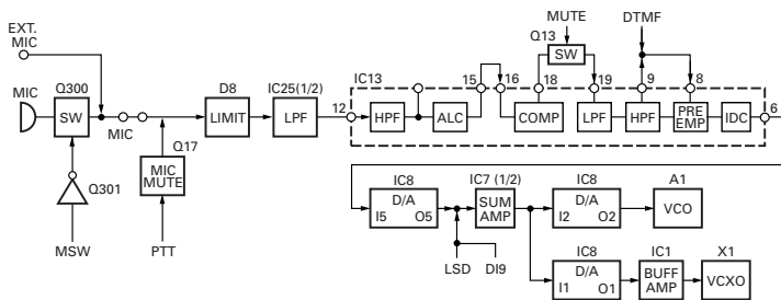
Fig. 7 Microphone amplifier
