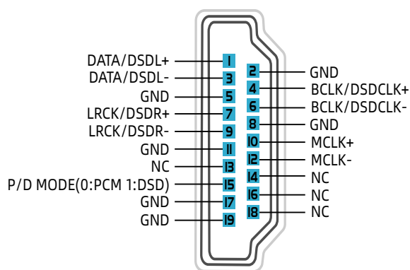
IIS OVER HDMI(Socket view)
