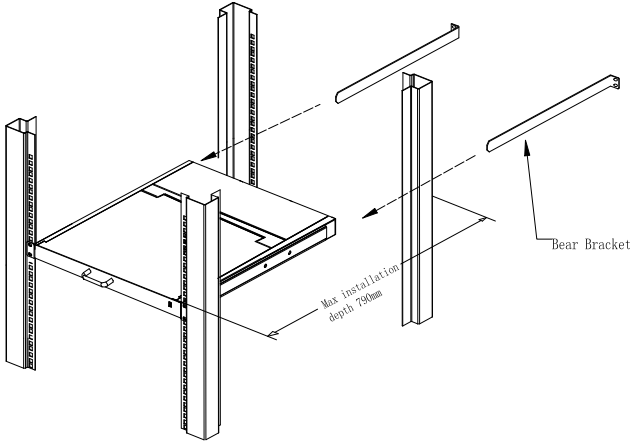
Figure2-1 rack mounting (1)
