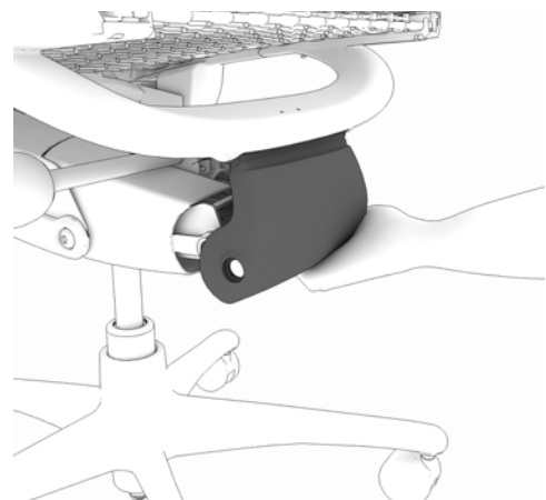
34. Pull lower cover forward to remove.
