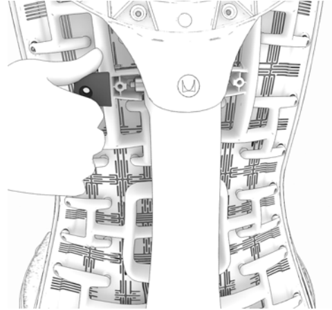
16. Remove hinge covers.
