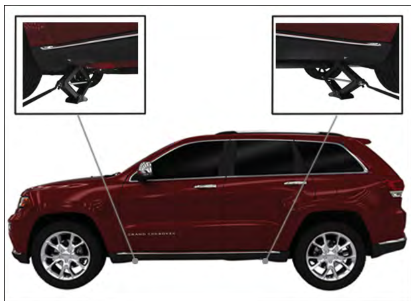
Jacking Locations
