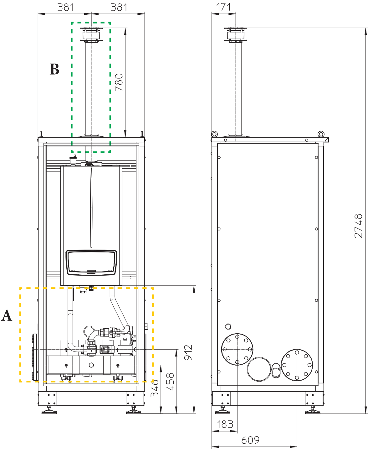
14.2 DIMENSIONS CABINET KIT + SINGLE VICTRIX PRO V2 35 - 55 - 60 - 68 - 80 EU
