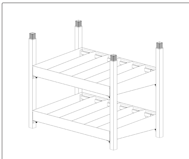
Step 8. Assembly complete.
