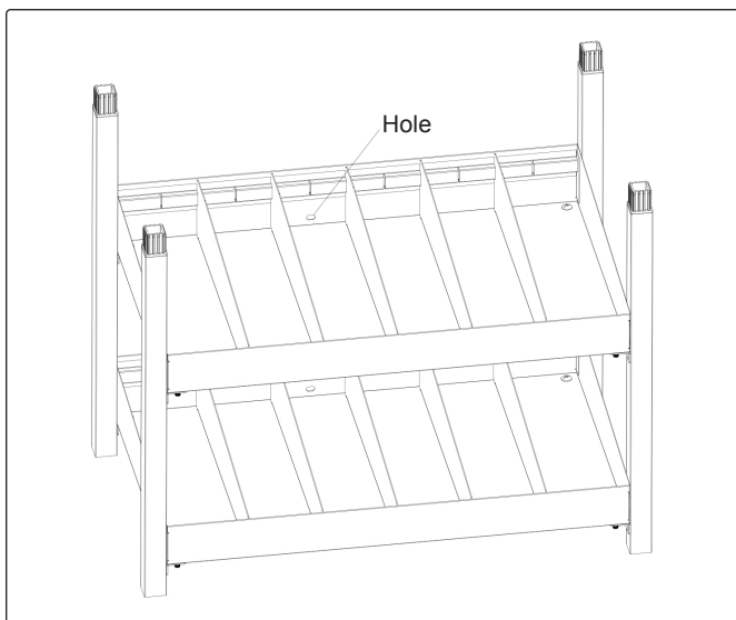
Step 3. To fix on the wall, mark the wall using the hole which is at the back of the tray.
