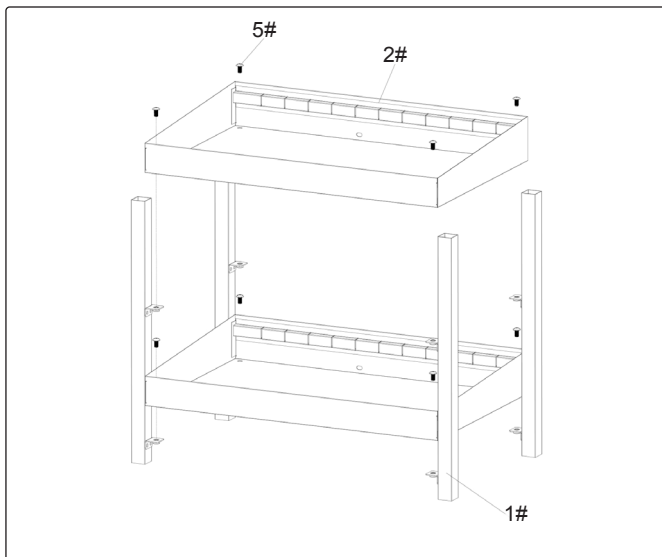
Step 1. Assemble the uprights, and fit the trays using M6*12 as shown.
