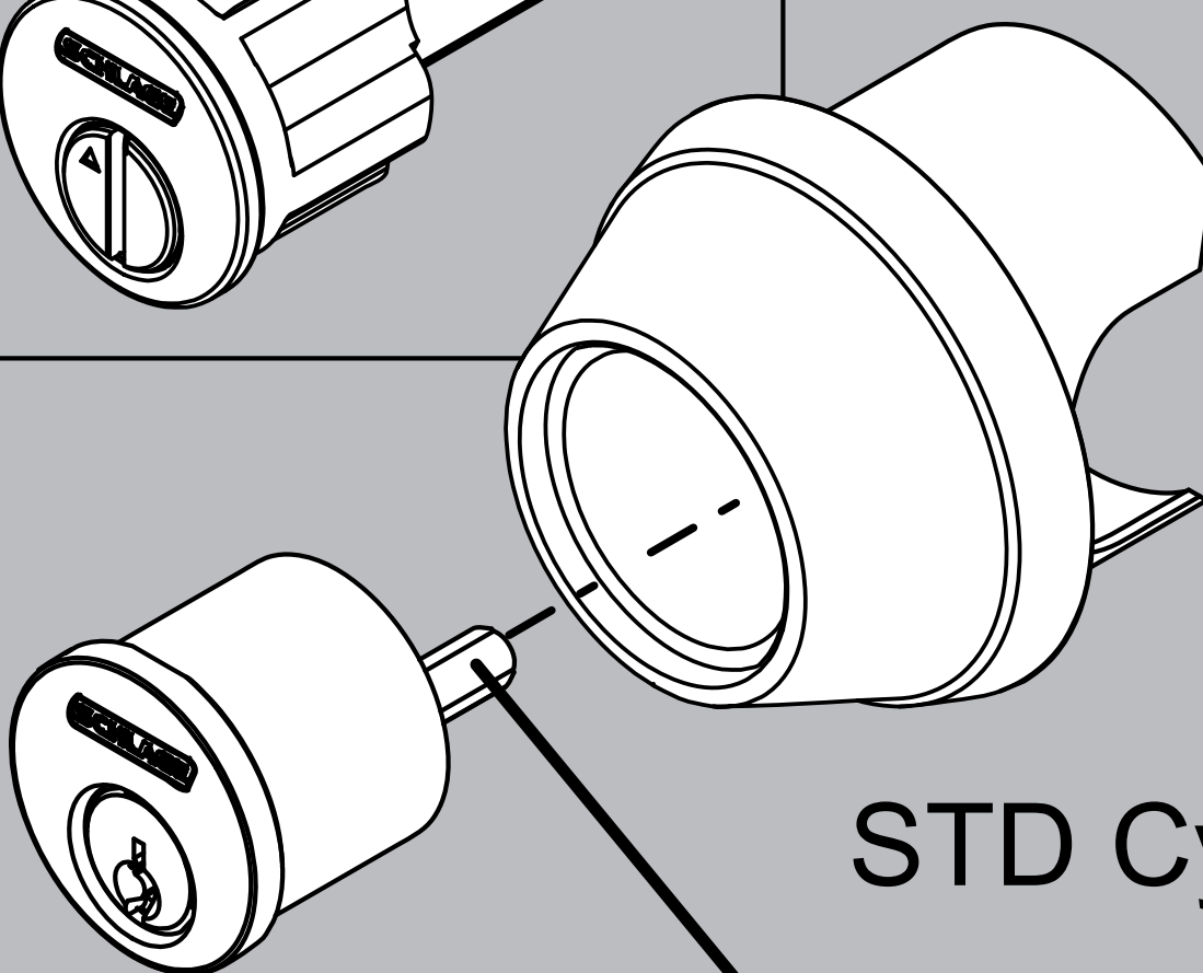
Drive bar
