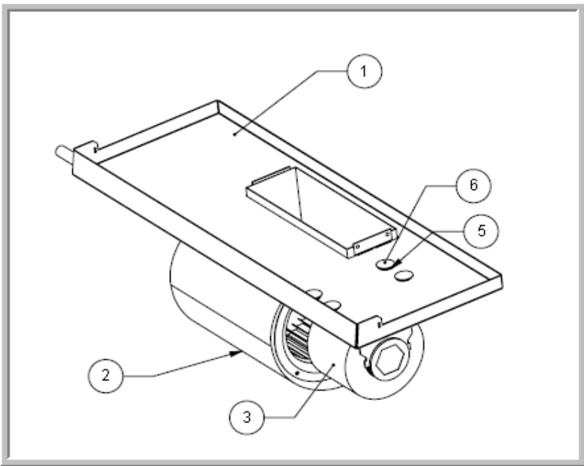
VF Series "B" Fan Deck Assembly
