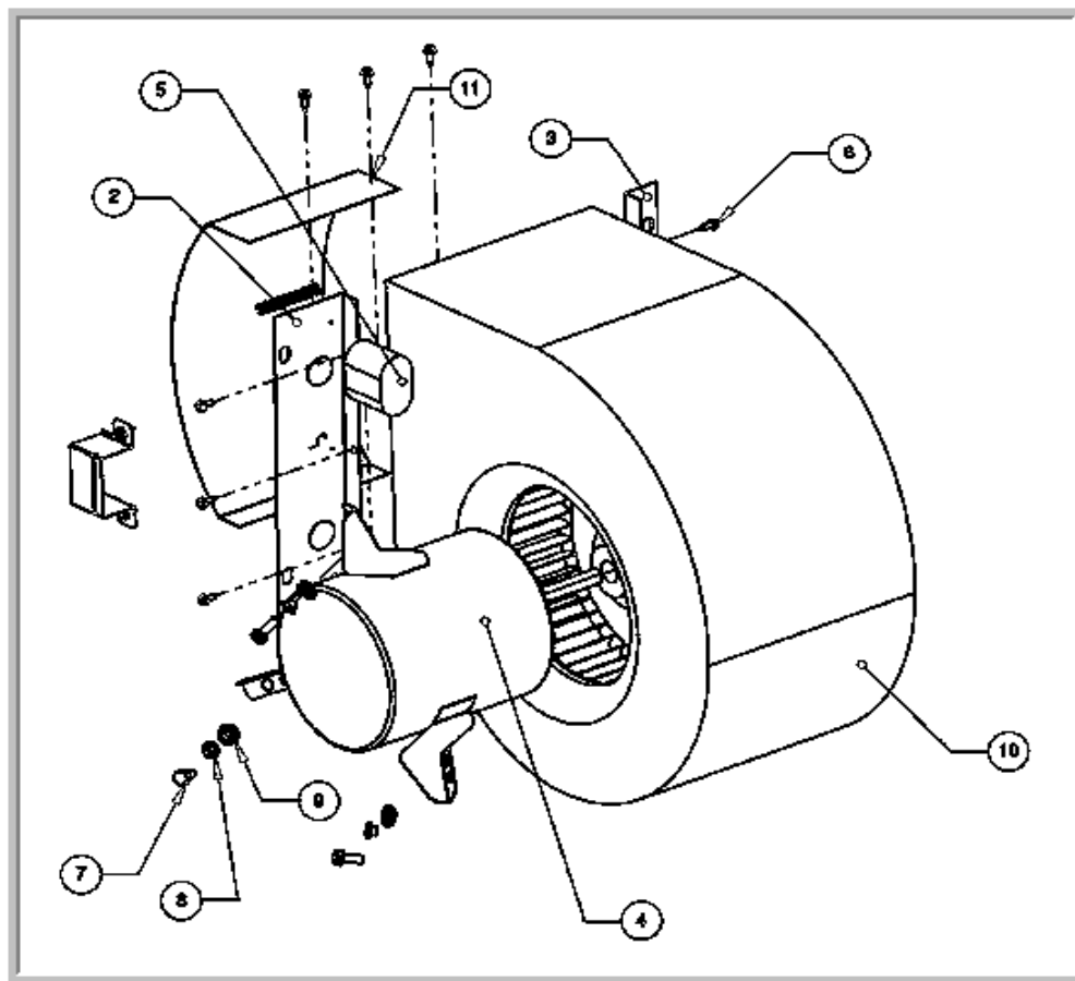
HP Fan Assembly with Fan Runners & Capacitor Bracket.
