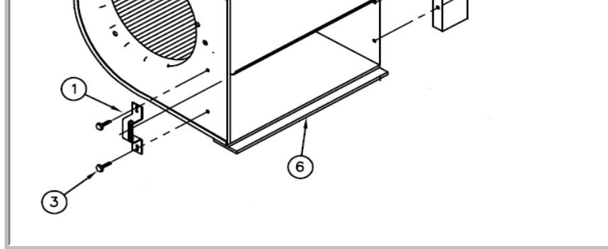
CDV & CDH Fan Assembly with Fan Runners, Capacitor Bracket and Guide Plate.
