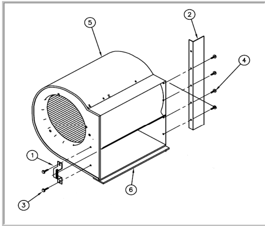
VH Fan Assembly with Fan Runners, Capacitor Bracket and Guide Plate.
