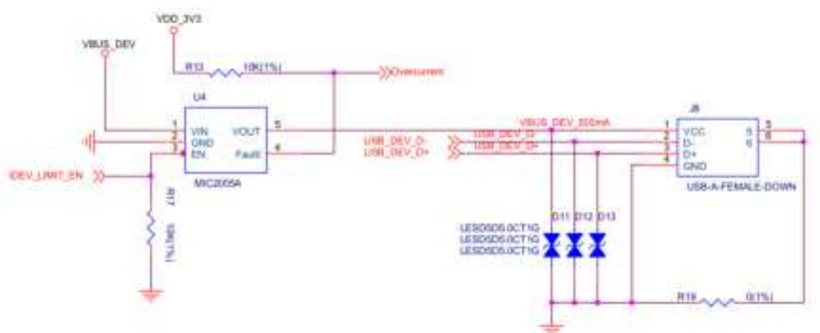
Fig. 10: 500 mA Current Limiting Circuit (click to enlarge)
