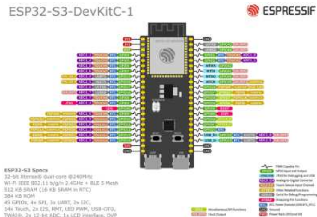
Fig. 4: ESP32-S3-DevKitC-1 Pin Layout (click to enlarge)
