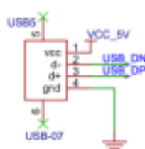
Fig. 6: ESP32-S3-USB-Bridge - Type-A Power Supply
