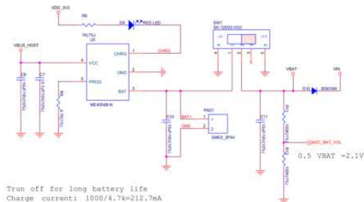
Fig. 14: Charging Circuit (click to enlarge)
