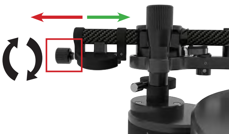
Pic. 21: Adjustment of the tracking force
