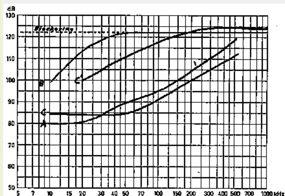
Fig 2. Two tone test of the receiver showing how strong an interfering signal can be (relative to the noise floor) without reducing the S/N of the desired weak signal with more than 3 dB. Curve A shows the performance in the original state. B shows a modified station. C and C' show another station before and after modification. (The MuTek front end board was used in all these tests)
