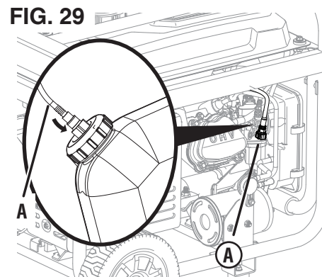
A - Injector hose
