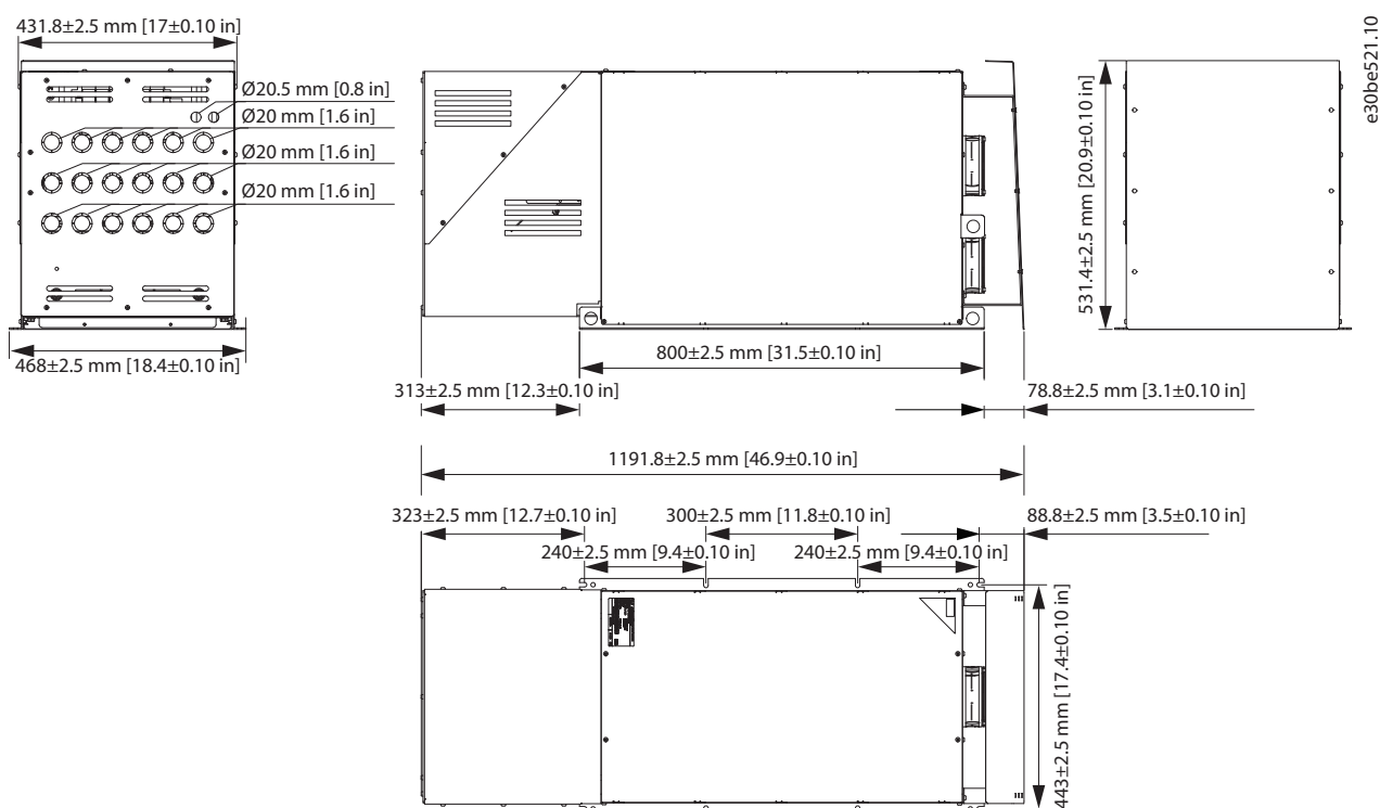
Illustration 7.48 IP21 X8-V3 Internal and External Fan
