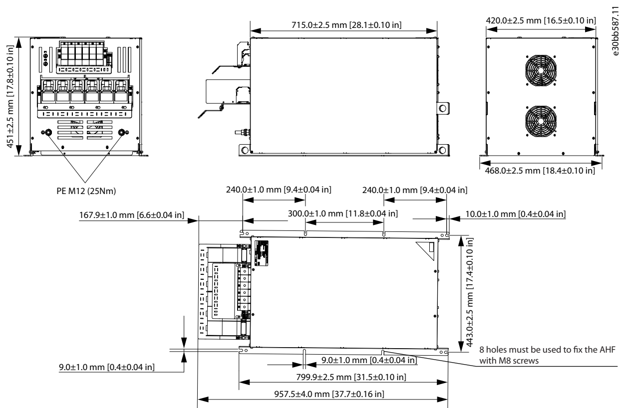
Illustration 7.26 IP20 X7-V3 Internal Fan
