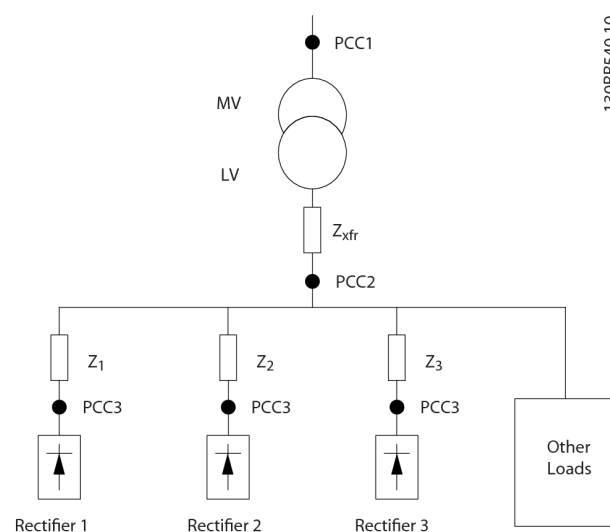
Illustration 2.4 Small Distribution System
