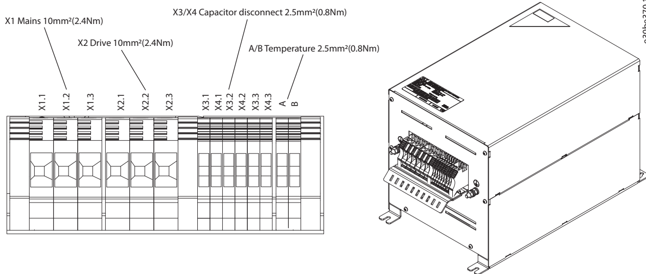
Illustration 7.9 IP20 X2-V3 External Fan, Terminal Designation and 3D View
