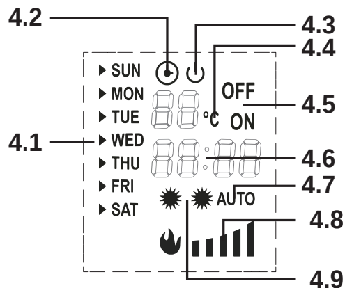
LCD-Display
