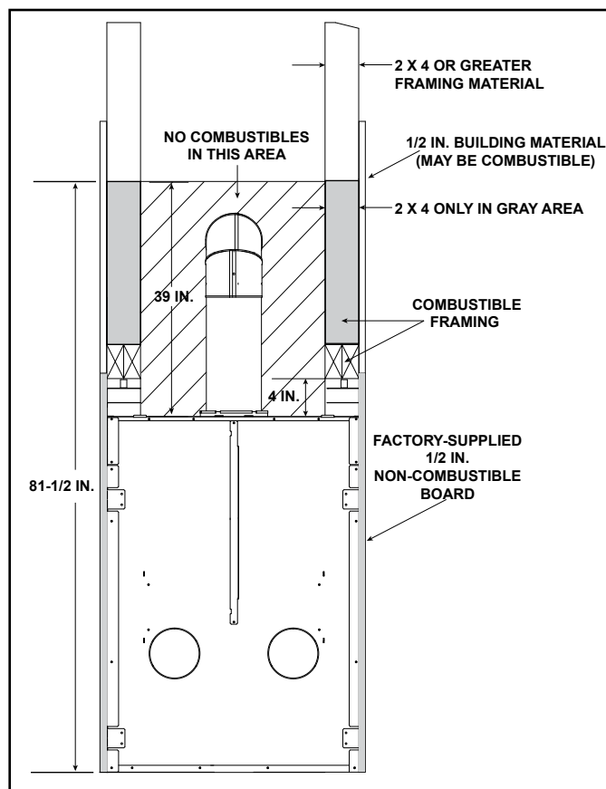
Figure 3.7 Non-Combustible Zone
