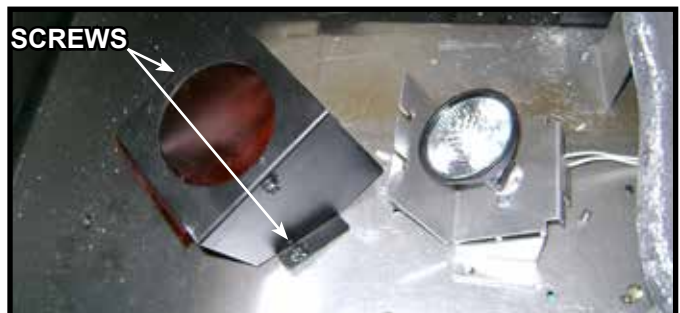
Figure 11.13 Light Housing Removed, Bulb Installed
