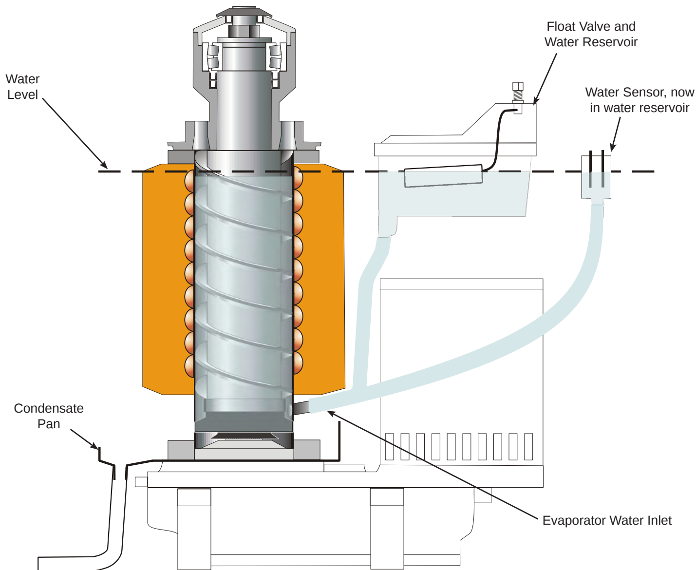
Water Schematic
