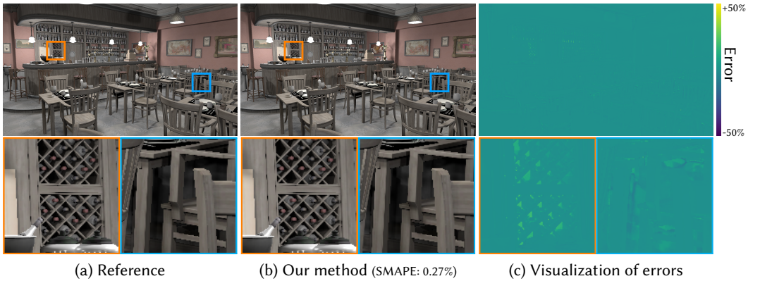
Fig. 11. ReSTIR with exact visibility test and our rejection method using 300000 samples per pixel for the BISTRO INTERIOR scene (1.3 M triangles, 44.0 k triangle lights). Our method produces a small bias in dark shadows as shown in the error visualization (c), but it is barely perceptible in the rendered image (b).
