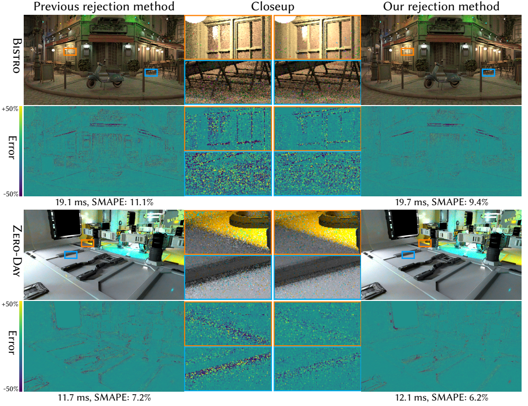
Fig. 10. ReSTIR with exact visibility test (5 rpp) for the BISTRO scene (2.8 M triangles, 20.6 k triangle lights) and the ZERO-DAY scene (5.2 M triangles, 10.3 k triangle lights). Although our rejection method introduces a small bias, it significantly reduces variance around shadow edges and material boundaries.
