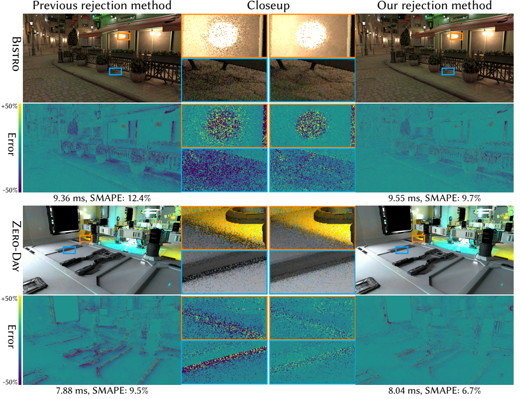
Fig. 5. Visibility-reuse ReSTIR with two rays per pixel (2 rpp) for the BISTRO scene (2.8 M triangles, 20.6 k triangle lights) and the ZERO-DAY scene (5.2 M triangles, 10.3 k triangle lights). Our rejection method reduces a darkening bias as well as variance on shadow edges. Our method also reduces variance around glossy highlights with temporal continuities.
