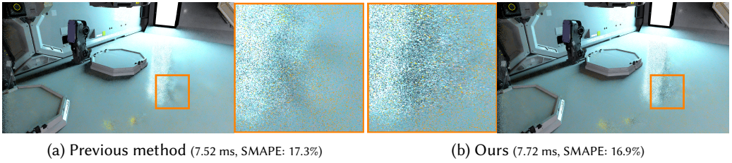
Fig. 13. Previous rejection method (a) and our rejection method (b) for glossy surfaces viewed from a moving camera (2 rpp). While our method reduces error on shadow edges, it can increase variance around glossy highlights as the camera moves. This is because our PDF shape estimation has a temporal delay when the view direction changes for glossy surfaces. Reduction of this delay is left for future work.
