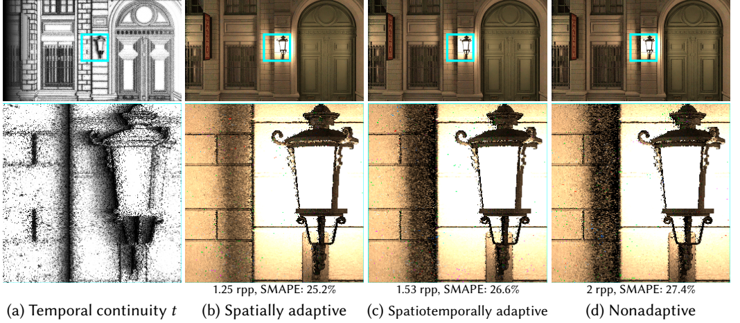
Fig. 9. Combination of our rejection method and adaptive shadow ray tracing for the BISTRO scene with a moving camera. Since our heuristic works only for temporally continuous pixels, (b) pixel-distance-based adaptive tracing [Wyman and Panteleev 2021] can lose shadows for temporal disocclusions. (c) We can compensate the lost shadows by tracing more shadow rays based on the temporal continuity, while this approach can increase a darkening bias as in 2-rpp nonadaptive tracing (d).
