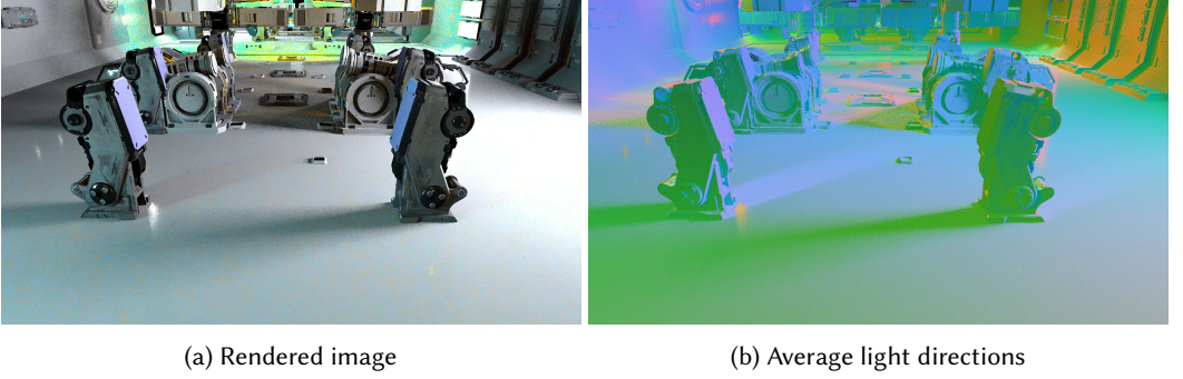
Fig. 3. Visualization of the estimated average light direction for each pixel. Average light directions are different between lit and shadowed pixels. By using these directions, we detect shadow edges for our rejection method.
