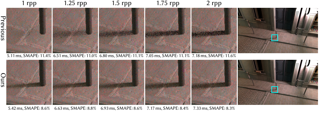
Fig. 8. Pixel-distance-based adaptive shadow ray tracing [Wyman and Panteleev 2021] with the previous rejection method (upper row) and our rejection method (lower row) for the BISTRO scene. Our method preserves more contact shadows than the previous method for a small number of rays per pixel (rpp).
