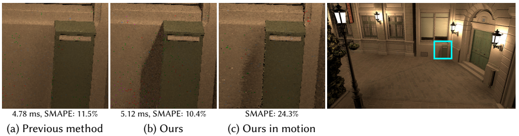
Fig. 7. Visibility-reuse ReSTIR with 1 rpp for a static camera (a, b) and moving camera (c) in the BISTRO scene. Although our heuristic (b) helps to render high-frequency shadows unlike the previous heuristic (a), it works only for temporal continuities. (c) For temporal discontinuities, our method uses the previous heuristic, and thus it can lose shadows in motion.
