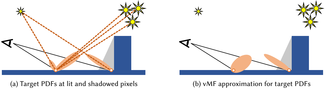
Fig. 2. (a) Target PDFs are different between lit and shadowed pixels for direct illumination. This paper rejects undesirable sample reuse across shadow edges by using the similarity of the PDF shapes. (b) To simplify the computation, we roughly approximate the target PDFs with vMF distributions in the light direction domain. Using this vMF approximation, we estimate the PDF similarity from the vMF lobe axes and sharpness.
