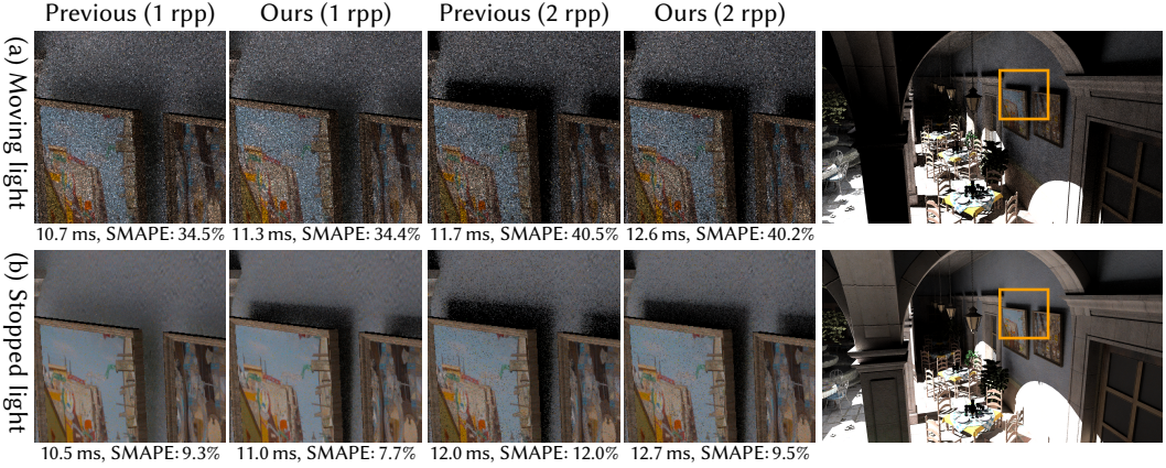
Fig. 12. Dynamic one-bounce indirect illumination from a point light source for the SAN MIGUEL scene (10 M triangles). (a) Our method produces comparable image quality to the previous method for a rapidly moving light source. (b) When the light source stops, our method renders higher-quality indirect shadows than the previous method.
