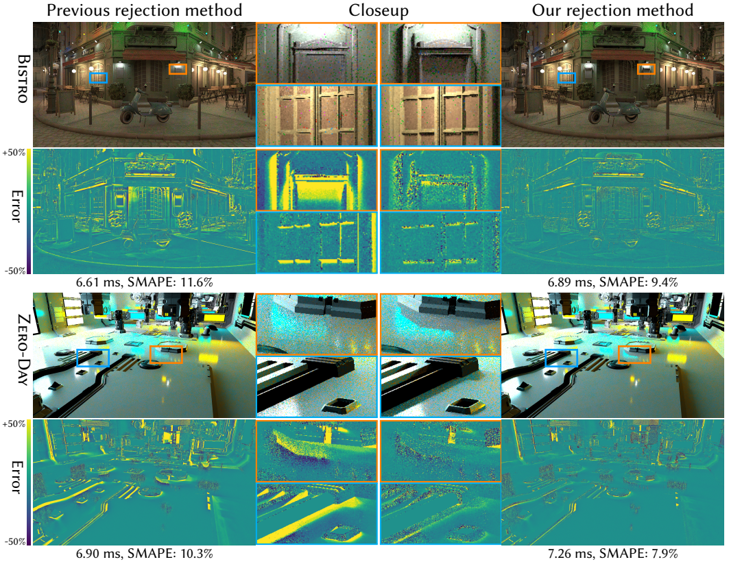
Fig. 6. Visibility-reuse ReSTIR with one ray per pixel (1 rpp) for the BISTRO scene (2.8 M triangles, 20.6 k triangle lights) and the ZERO-DAY scene (5.2 M triangles, 10.3 k triangle lights). While the previous rejection method loses hard contact shadows, our method reduces the loss of these high-frequency shadows.
