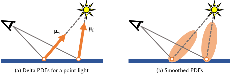
Fig. 4. PDFs are delta functions for a point light source (a). Although the PDF similarity between pixels can be obtained using the product integral of PDFs, it is always zero for delta PDFs since we ignore the shift of light directions. For such shifted high-frequency PDFs, we use the similarity of smoothed PDFs (b).
