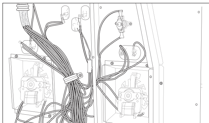
Figure 4-12. Limit Switch Removal.
