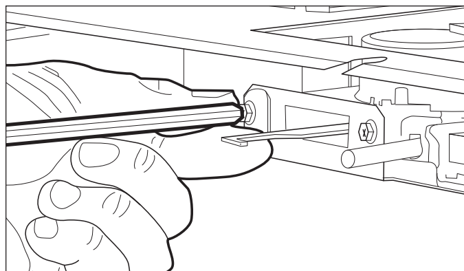
Figure 4-10. Motorized Door Latch Removal.
