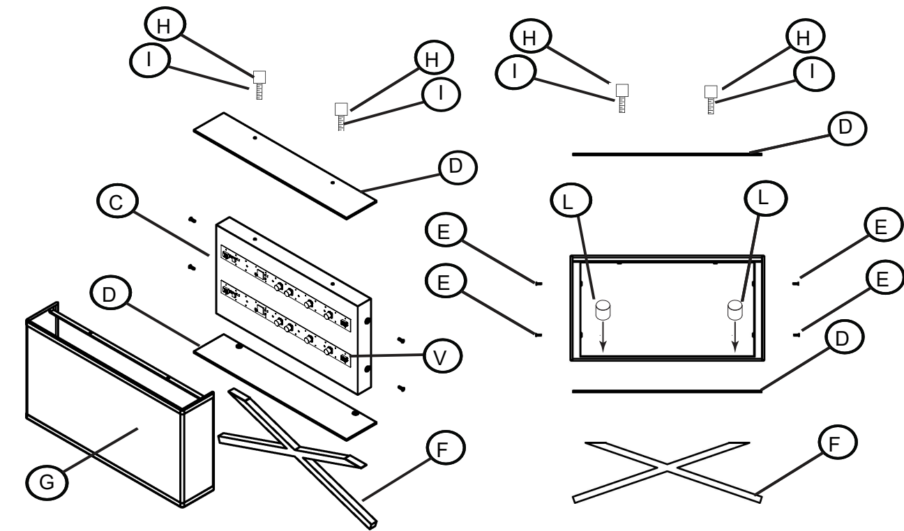
DRAWING 2- JUNCTION BOX MOUNTING
