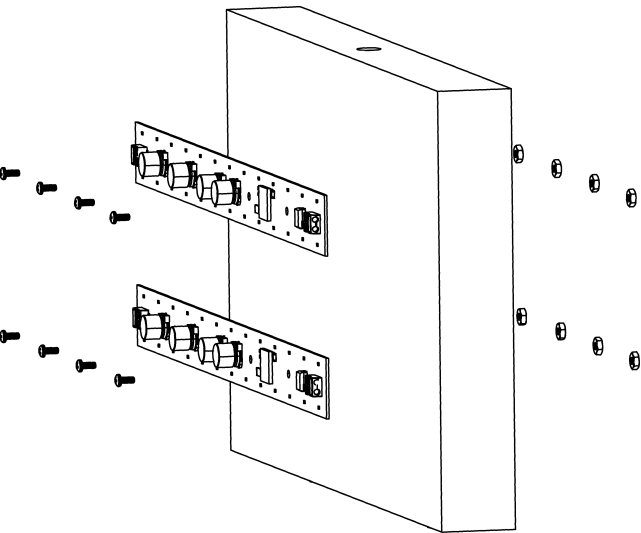
DRAWING 2 - LED REPLACEMENT
