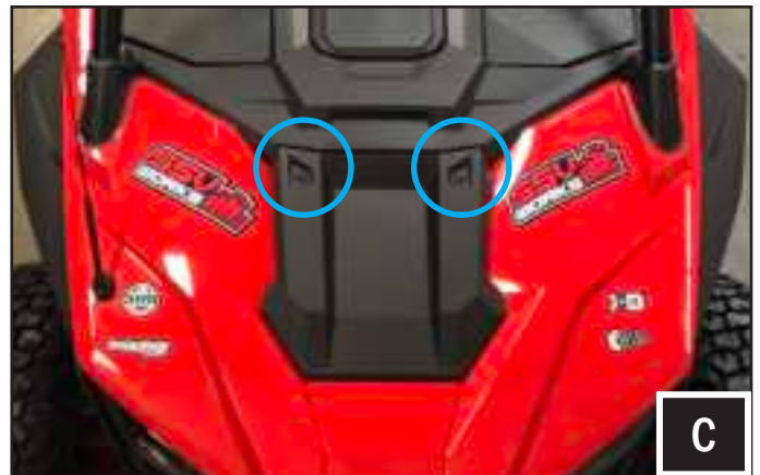
C. Remove the (2) T40 torx screws and set the hood panel aside.
