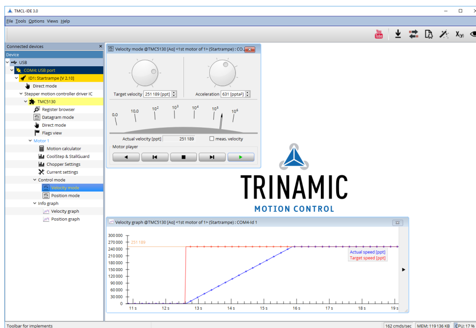
Figure 4: Driving the motor in velocity mode (TMCL-IDE provides similar view for TMC2160-EVAL)
