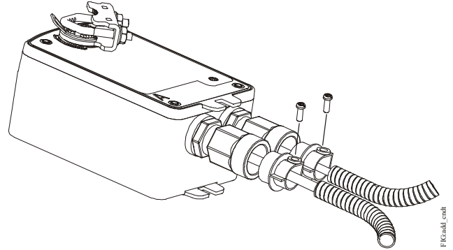
Figure 11: Adding Flexible Metal Conduit
