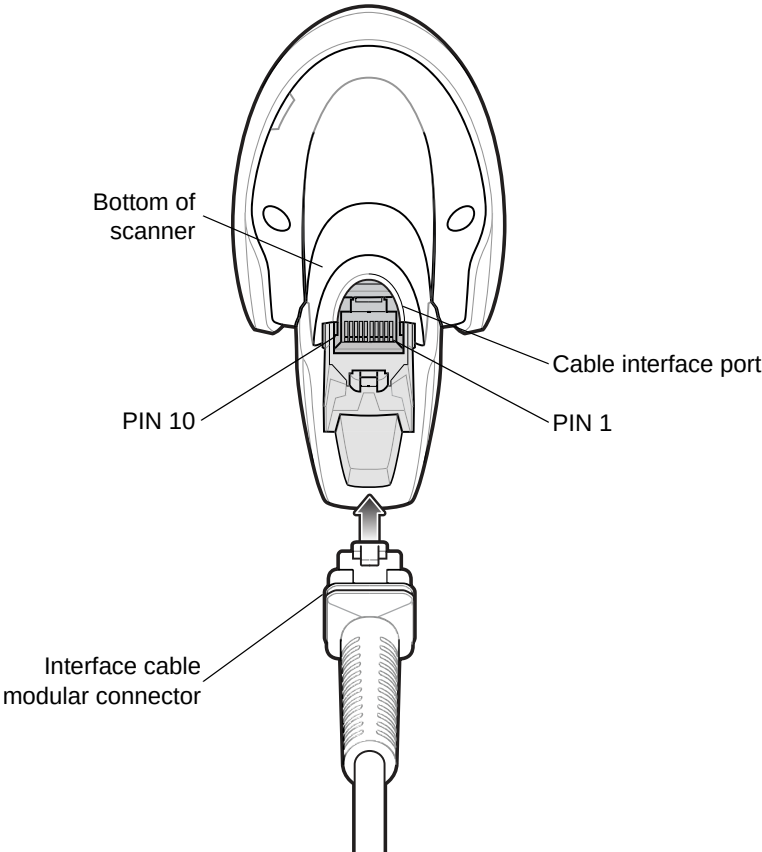
Figure 3-1 Digital Scanner Cable Pinouts
