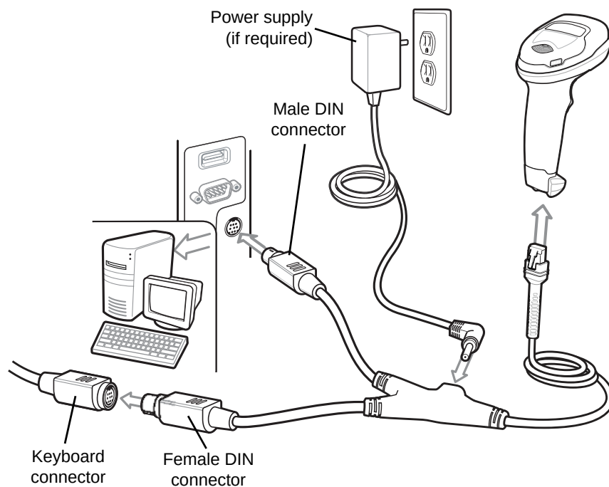
Figure 9-1 Keyboard Wedge Connection
