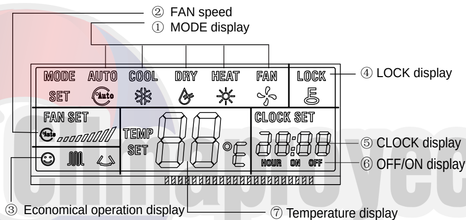
Name and function of LCD display on the wired controller
