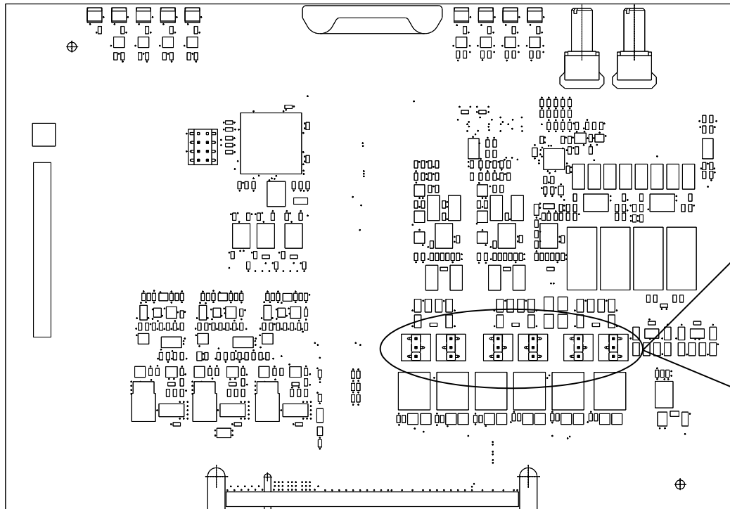
Figure 2 Jumpers on VCC2002-A1 voice I/O Card
