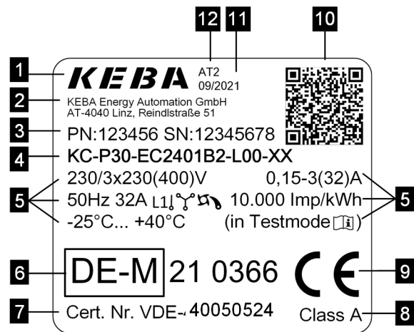
Fig. 3-2: Example type plate
