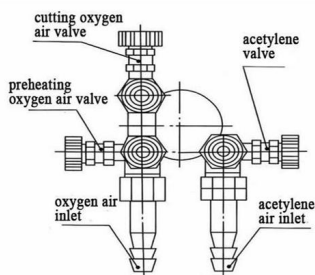
Gas distributor
