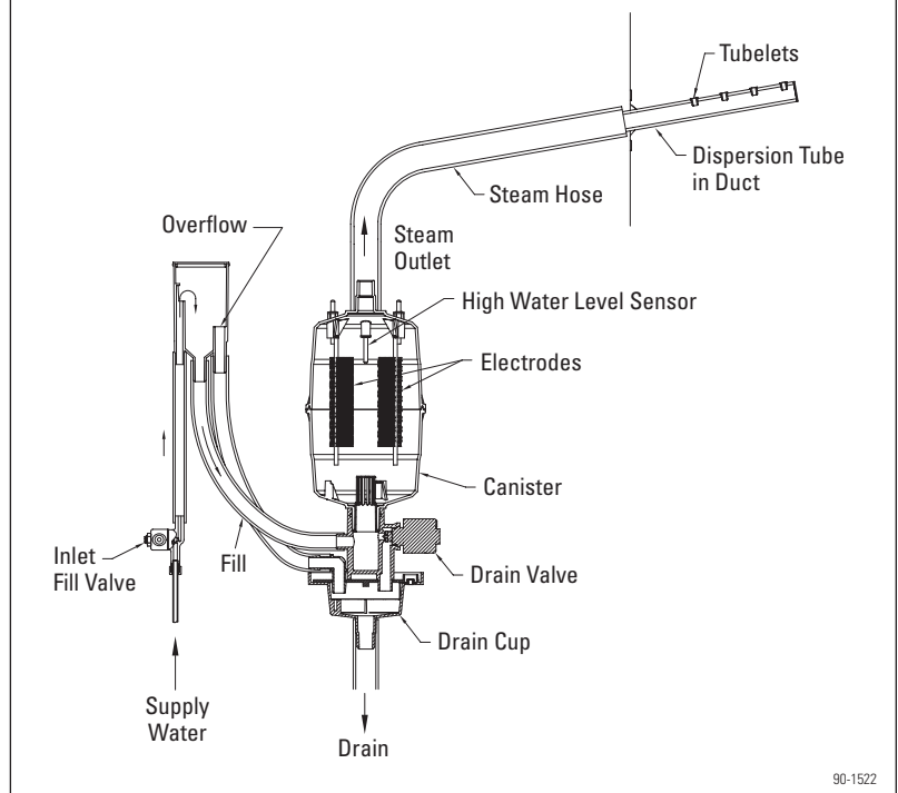
FIGURE 1 – Fill and Drain System and Canister
