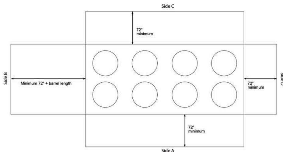
Figure 2. Recommended chiller clearances
