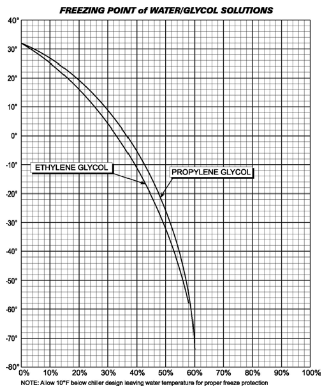
Figure 35. Water/Glycol concentration freezing points (in degrees Fahrenheit)
