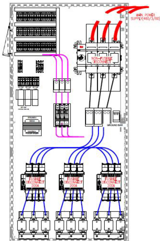
Figure 5. Power panel
