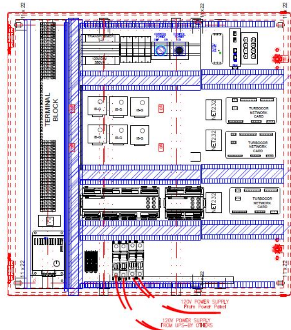
Figure 6. Control panel
