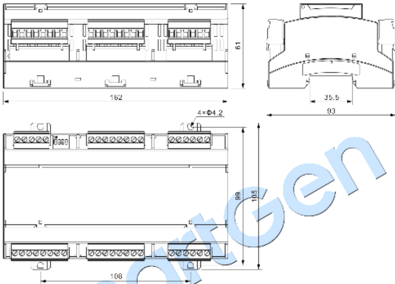
Fig.2 Case Dimensions
