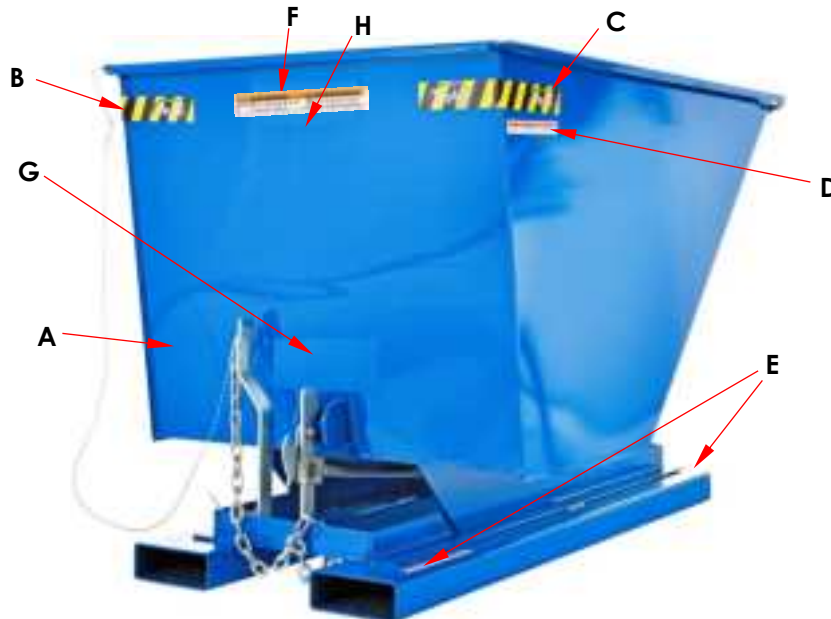
B: Label 1037 (CAUTION on side of hopper)
