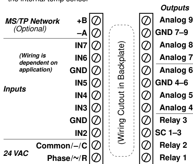
Illustration 6—BAC-19xx36 Terminals and Connections
