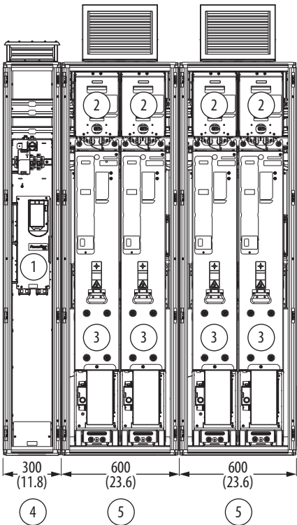
Left-to-Right Orientation Enclosures are 600 mm (23.6 in.) deep. IP54, UL Type 12 Enclosure Shown.
