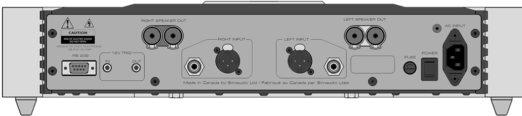
Figure 1: 760A Backpanel
