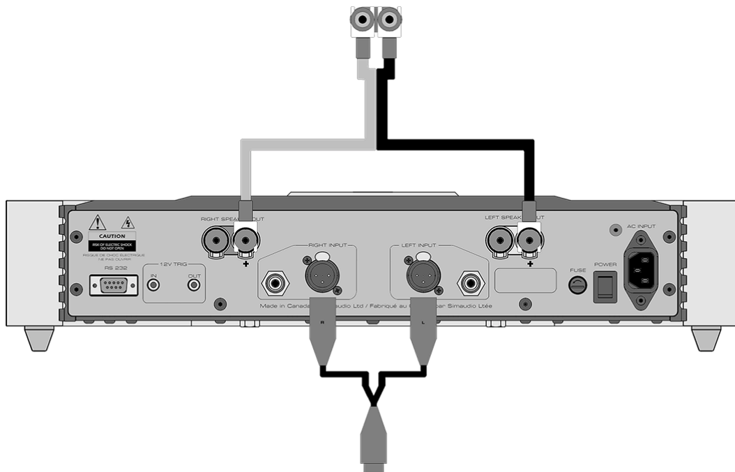
Figure 3: Bridged-Mono operation of the MOON 760A Power Amplifier
