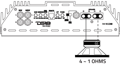
SPEAKER CONNECTION 1
