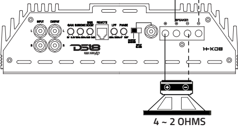
SPEAKER CONNECTION 2
