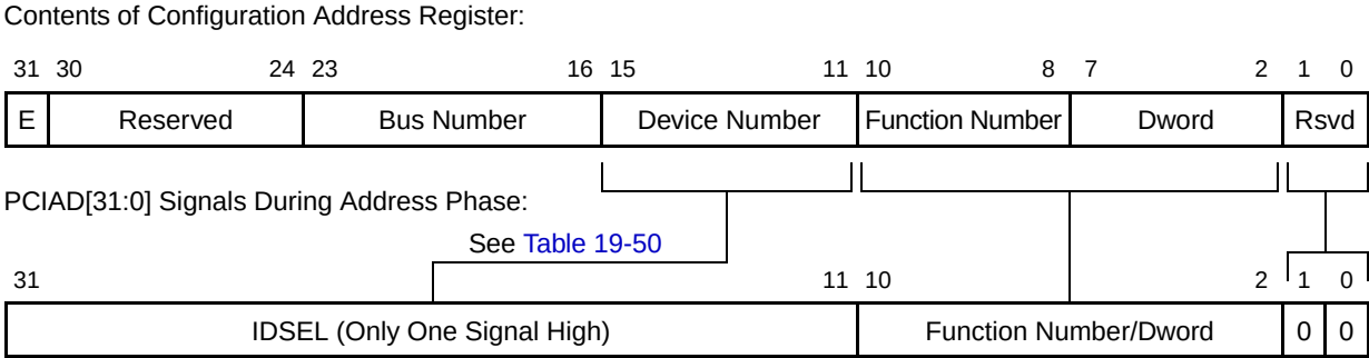
Figure 19-53. Type 0 Configuration Translation
