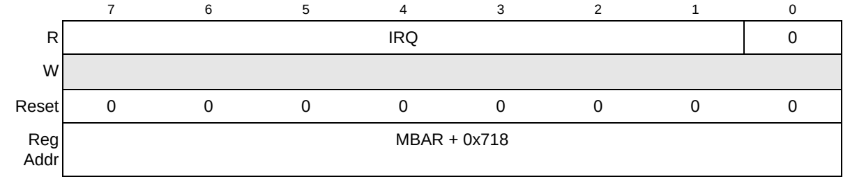
Figure 13-7. Interrupt Request Level Register (IRLR)
