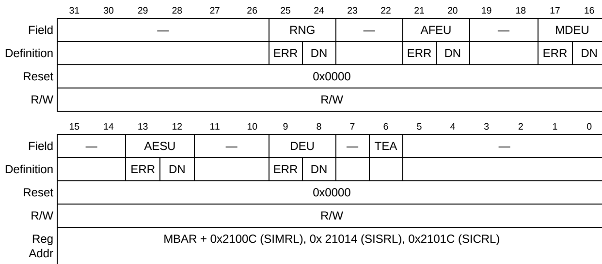
Figure 21-12. SEC Interrupt Mask, Status, and Control Registers Low (SIMRL, SISRL, and SICRL)
