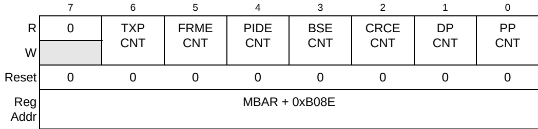
Figure 29-25. USB Counter Overflow Register (CNTOVR)
