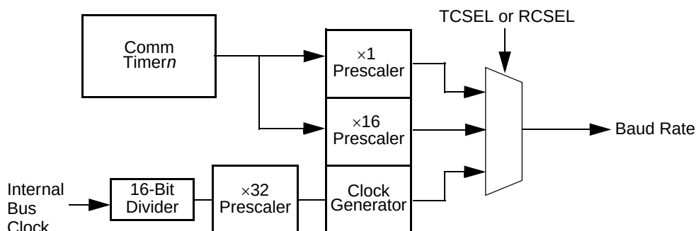
Figure 26-5. UART and SIR Baud Rate Clocking Sources
