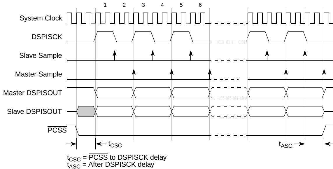
Figure 27-18. DSPI Modified Transfer Format (MTFE = 1, CPHA = 1, Fscck = Fsys/4)
