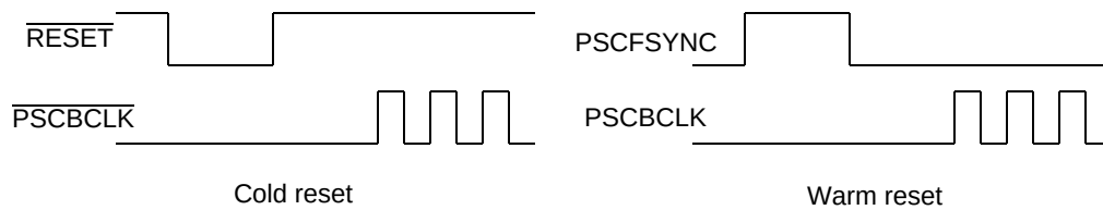
Figure 26-43. AC97 Cold and Warm Reset
