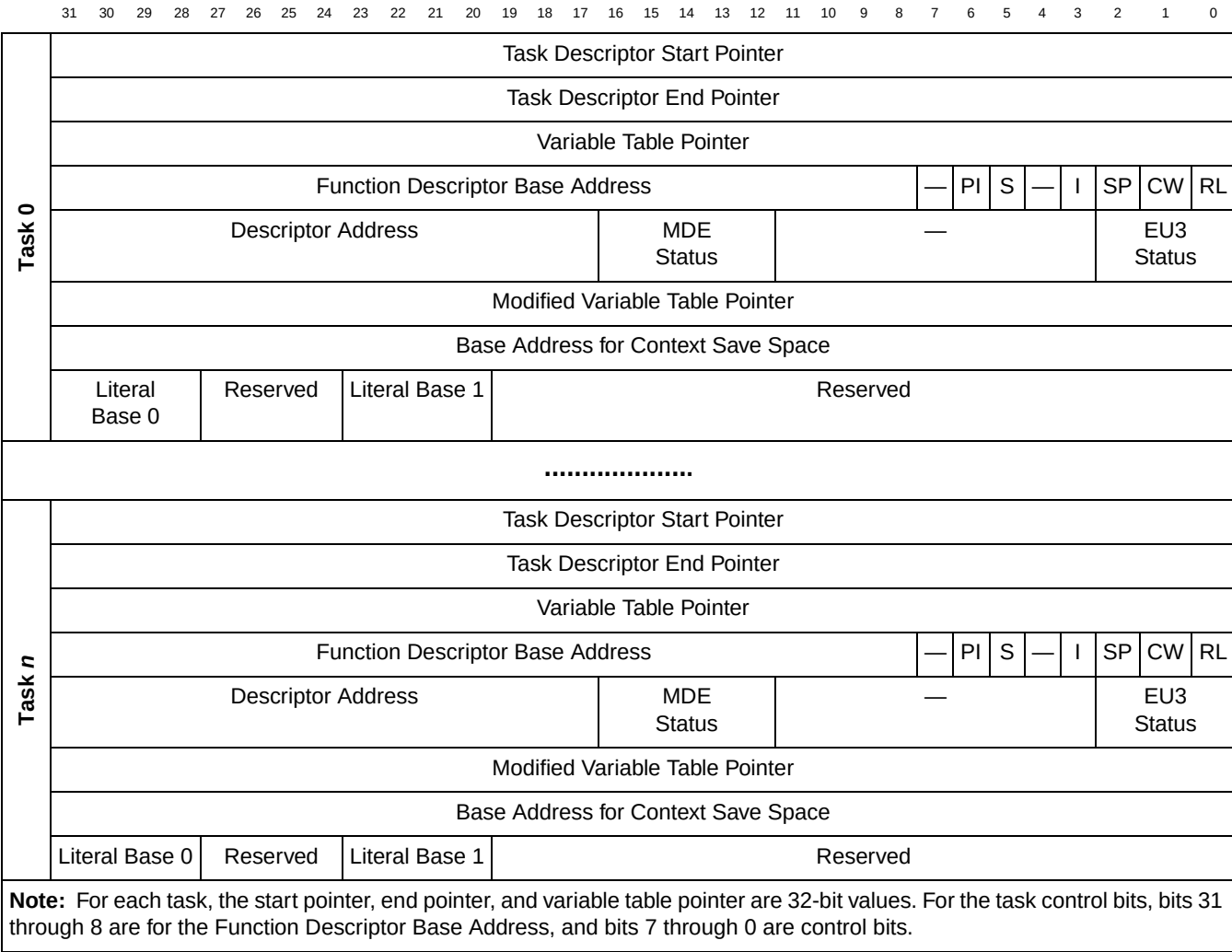
Figure 23-23. Task Descriptor Table Format
