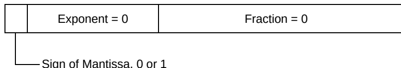
Figure 6-4. Zero Format
