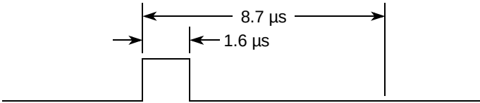
Figure 26-47. Serial Interaction Pulse (SIP)
