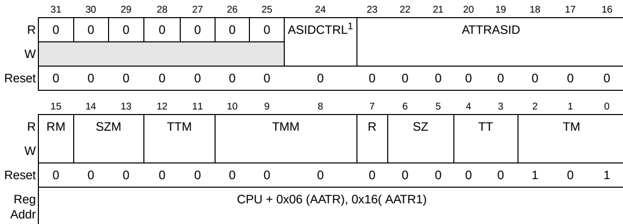
Figure 8-9. Address Attribute Trigger Registers (AATR, AATR1)
