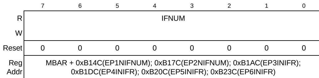
Figure 29-31. Endpoint n Interface Number Register IN (EP n INIFR)
