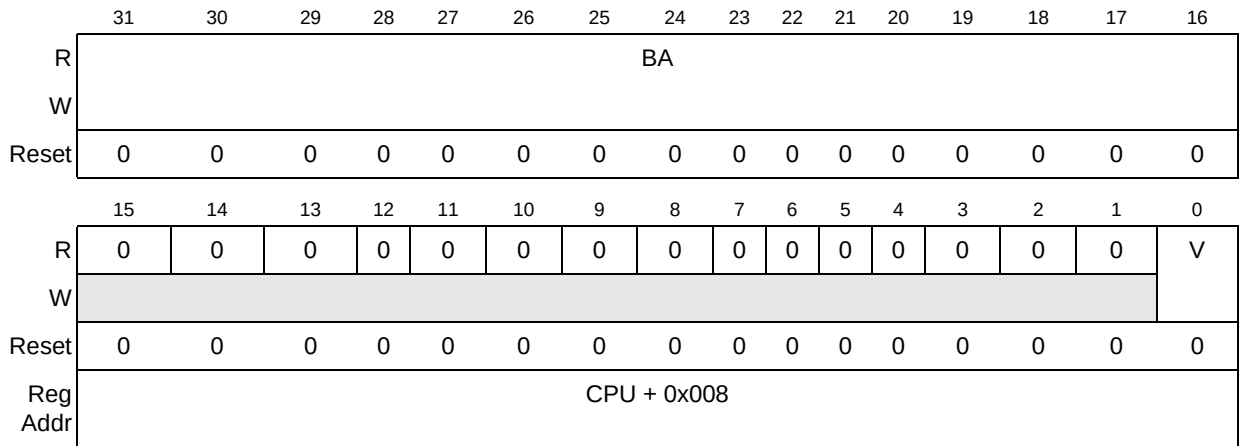
Figure 5-3. MMU Base Address Register (MMUBAR)
