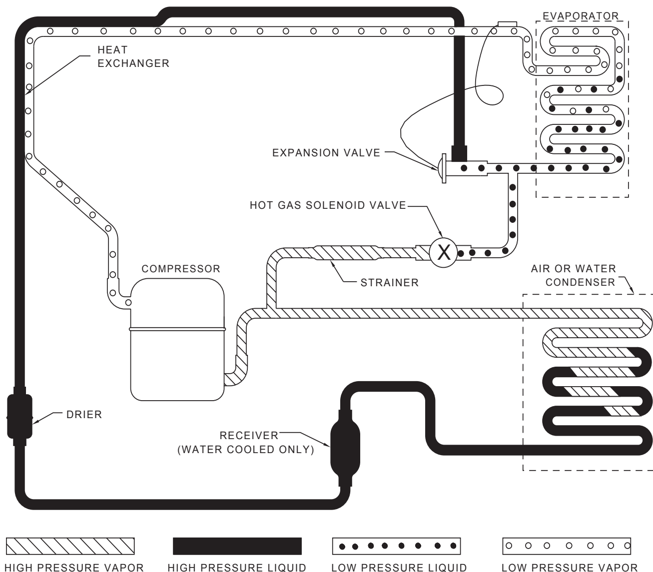
Figure 7-1. Self-Contained Prechill and Freeze Cycle
