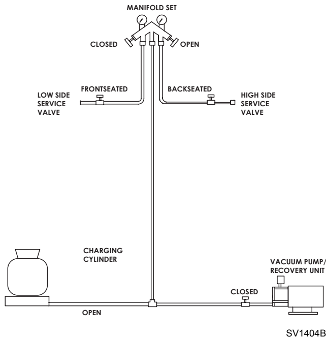
Figure 7-8. Charging Connections
