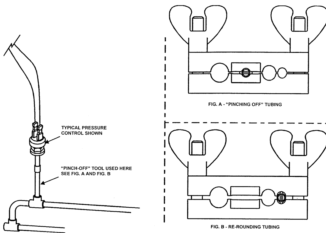
Figure 7-10. Using Pinch-Off Tool
