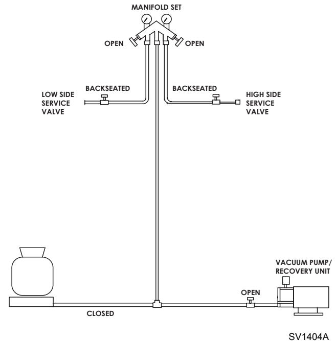
Figure 7-7. Recovery/Evacuation Connections
