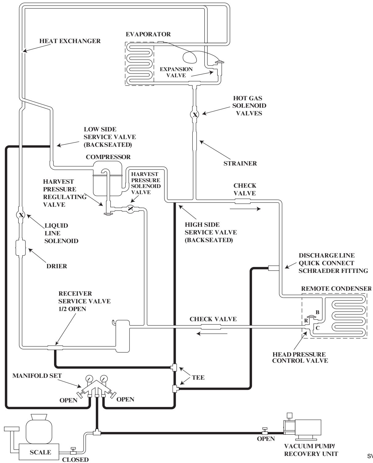
Figure 7-9. Recovery/Evacuation Connections
