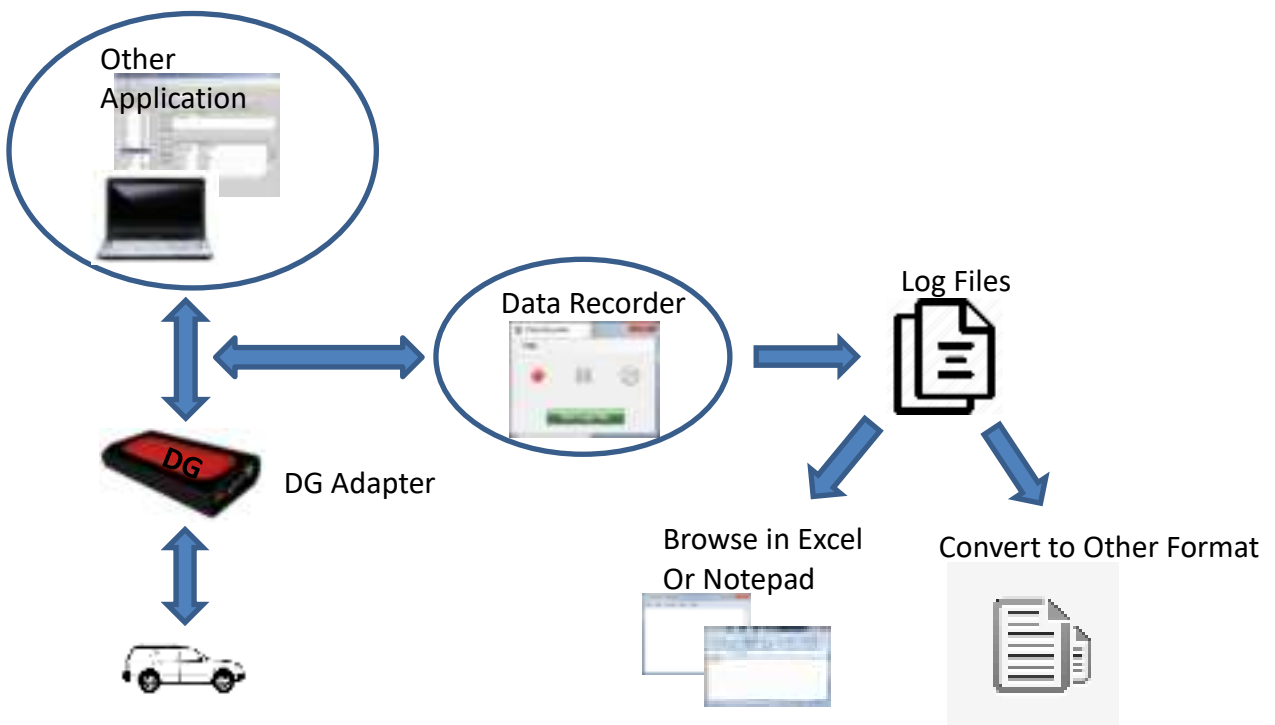
Figure 3 - Dependency Mode
