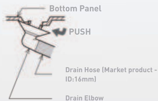
Figure 7: How to attach drain elbow.
