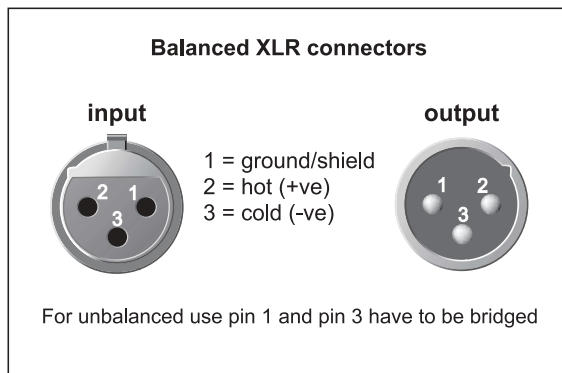
Fig. 4.1: XLR connections
