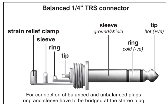
Fig. 4.3: 1/4" stereo plug
