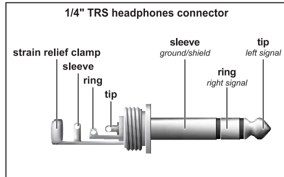
Fig. 4.4: Stereo plug for headphones connection
