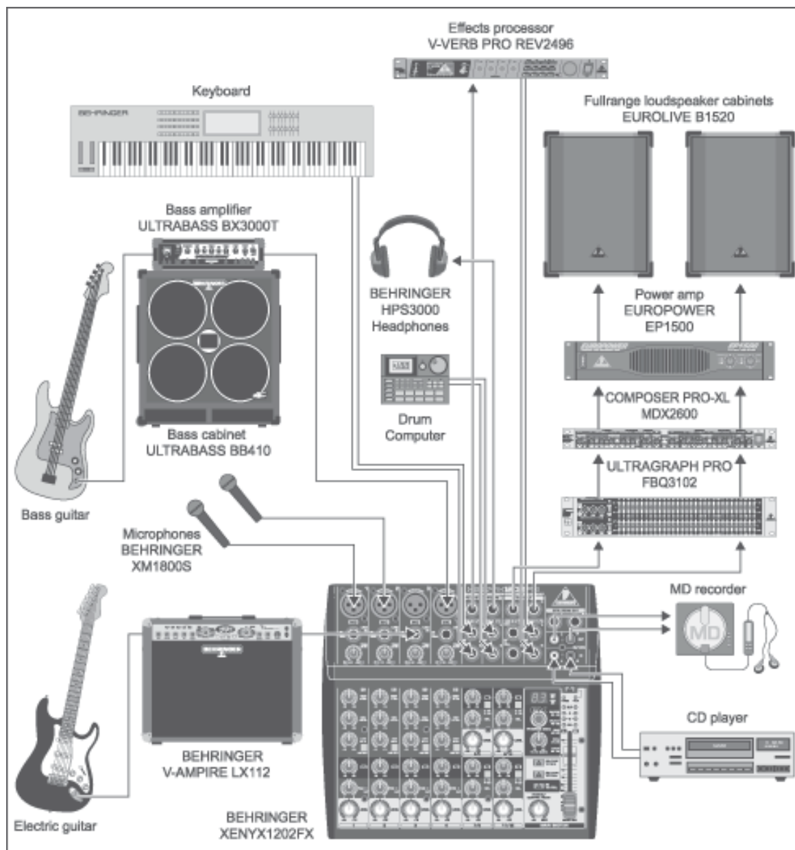
Fig. 3.2: Live application of the 1202FX
