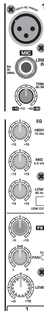
Fig. 2.1: Connectors and controls on the mono channels
