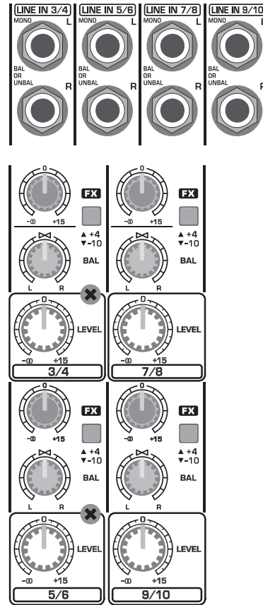
Fig. 2.2: Connectors and controls on the stereo channels
