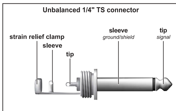
Fig. 4.2: 1/4" mono plug
