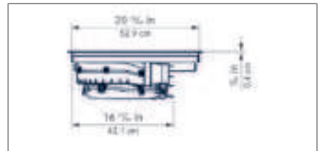
Fig. 5.3 Appliance dimensions side view
