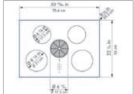
Fig. 5.1 Appliance dimensions top view
