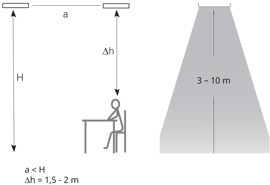
Fig.2. Positioning
