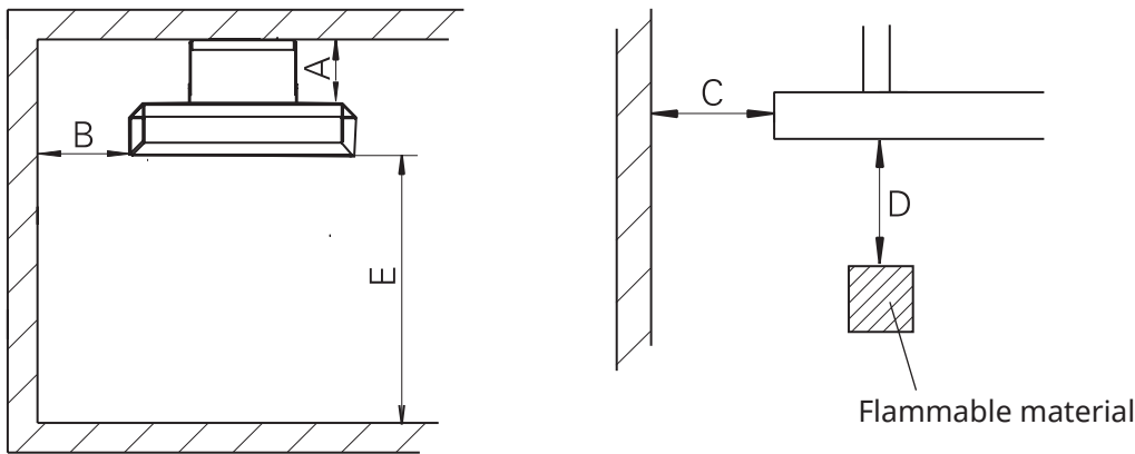
Fig.3. Minimum distances
