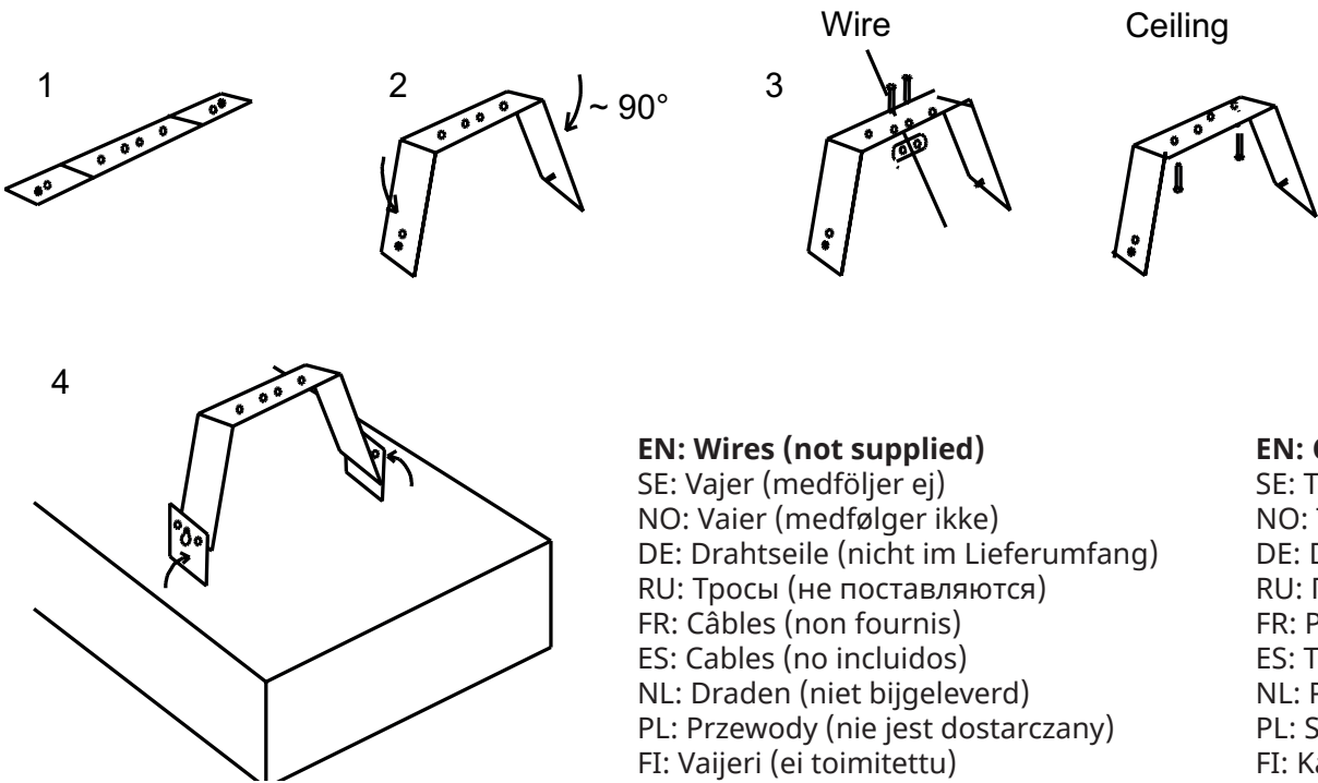
Fig.1. Mounting
