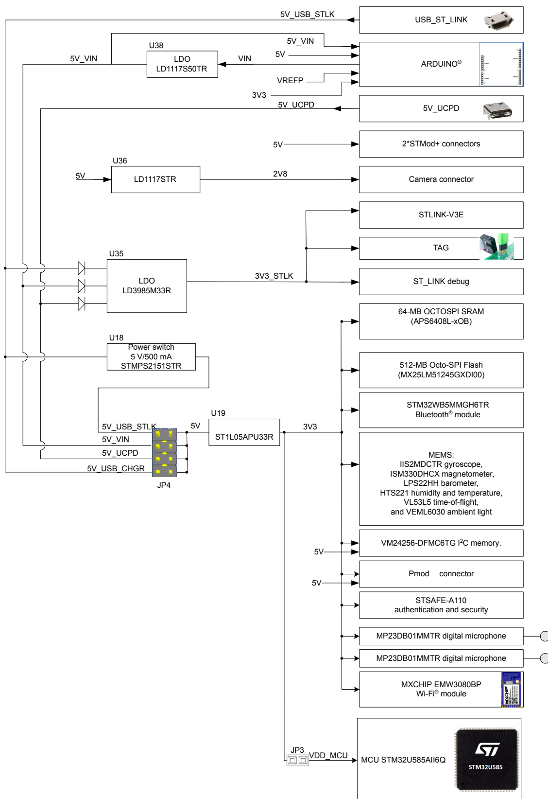
Figure 14. Power tree
