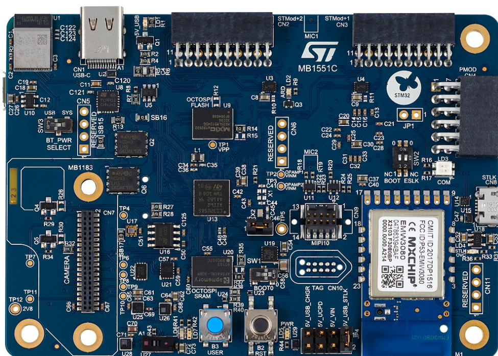
Figure 1. B-U585I-IOT02A Discovery kit for the IoT node
