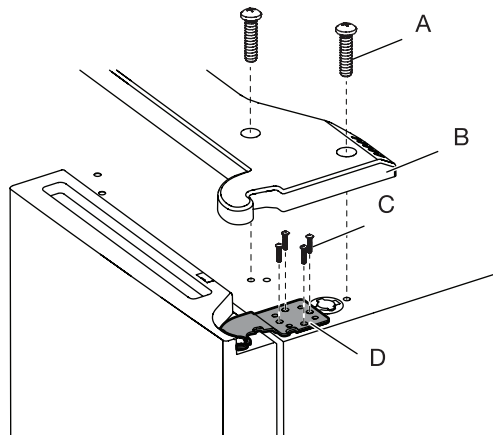
A. Top hinge cover screw B. Top hinge cover C. 5 mm socket screws D. Top hinge
